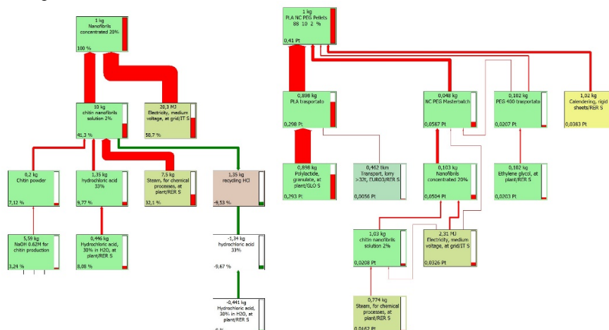
Figure 2. Net scheme of production of PLA/NC/PEG400 pellets
